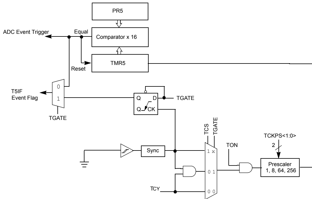
FIGURE 11-3: 16-BIT TIMER5 BLOCK DIAGRAM
