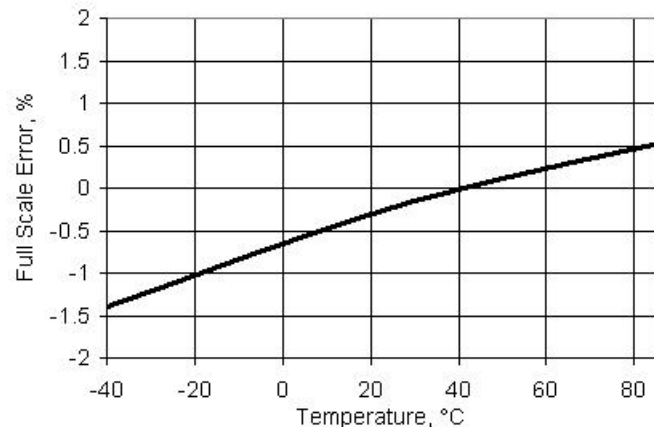
Figure 11-28. IDAC Full Scale Error vs Temperature, Range = 255 \mu A, Source Mode
