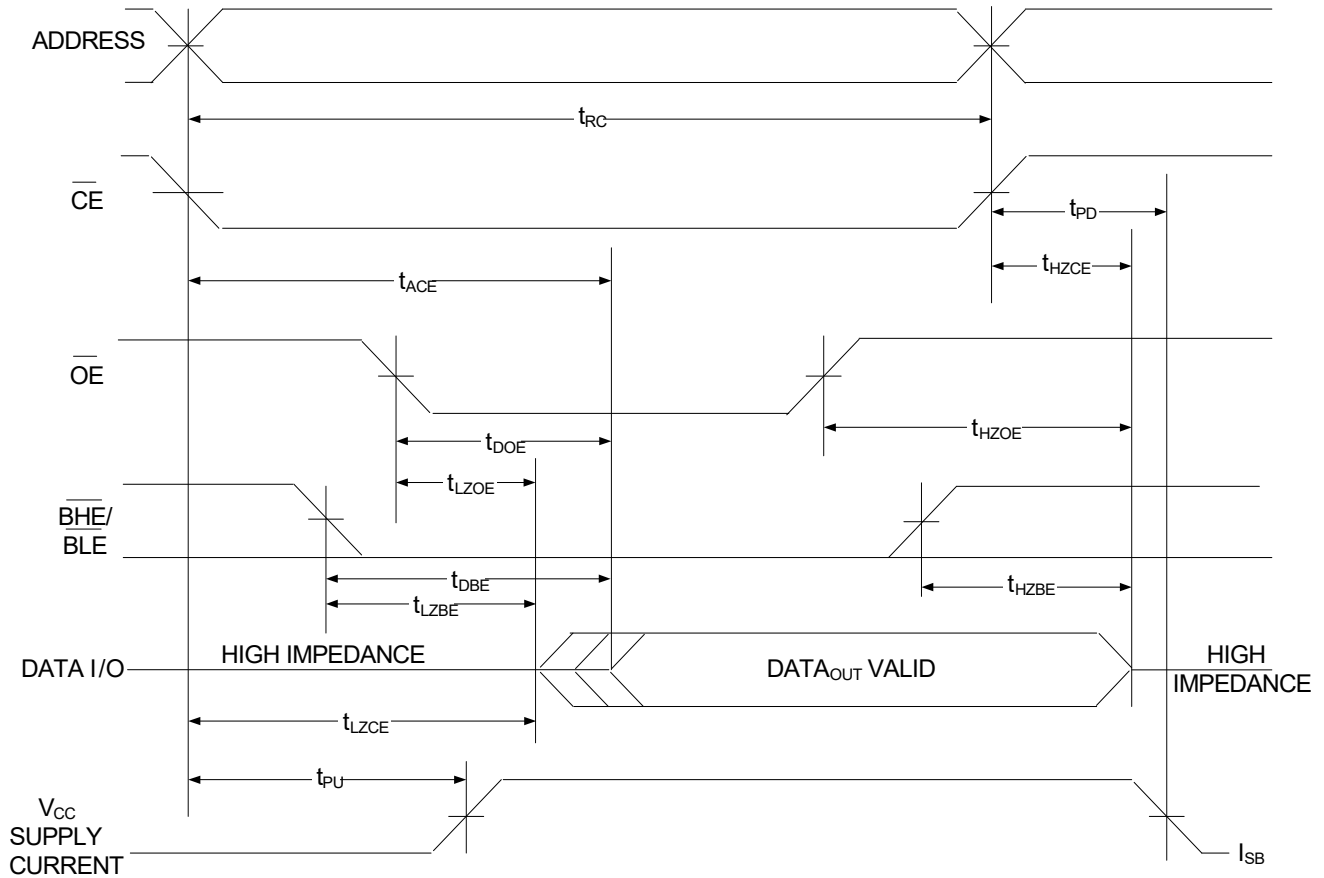
Figure 11. Read Cycle No. 2 ( \overline{OE} Controlled) [24, 25]
