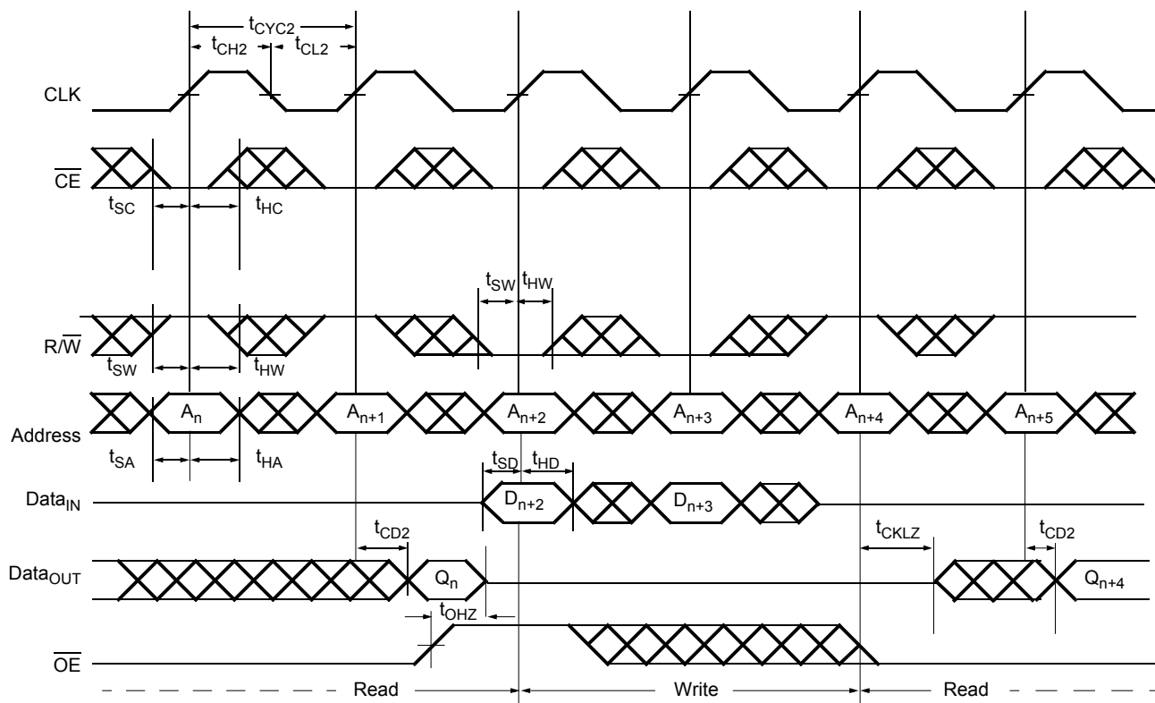
Figure 11. Pipelined Read-to-Write-to-Read ( \overline{OE} Controlled) [31, 32, 33, 34]
