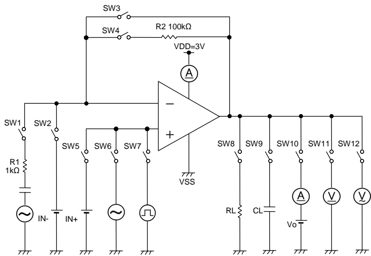
Figure 26. Test Circuit 2
