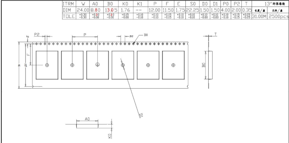
Figure 18: Tape specifications
