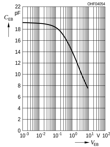
Emitter-Base Capacitance 1) page 11 Emitter-Basis Kapazität 1) Seite 11 C_{EB} = f(V_{EB}), f = 1 \text{ MHz}, E = 0
