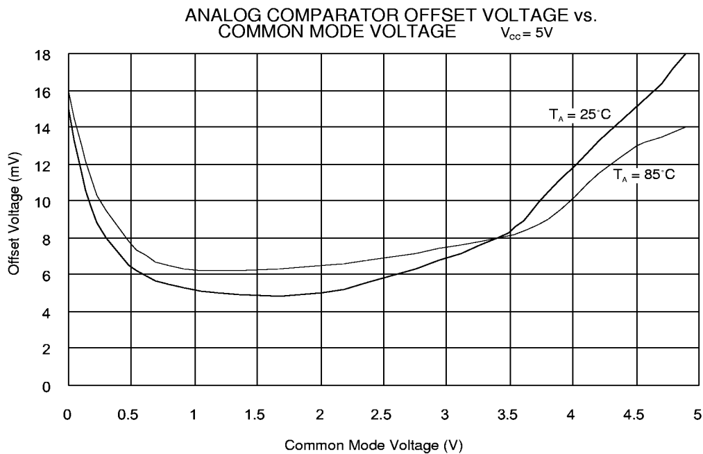
Figure 76. Analog Comparator Offset Voltage vs. Common Mode Voltage
