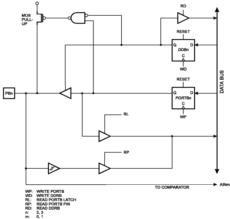
Figure 47. Port B Schematic Diagram (Pins PB2 and PB3)
