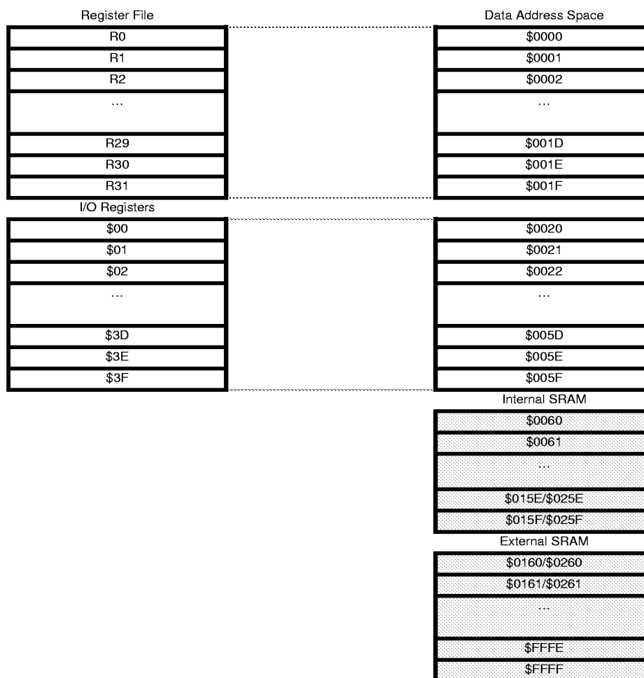
Figure 8. SRAM Organization
