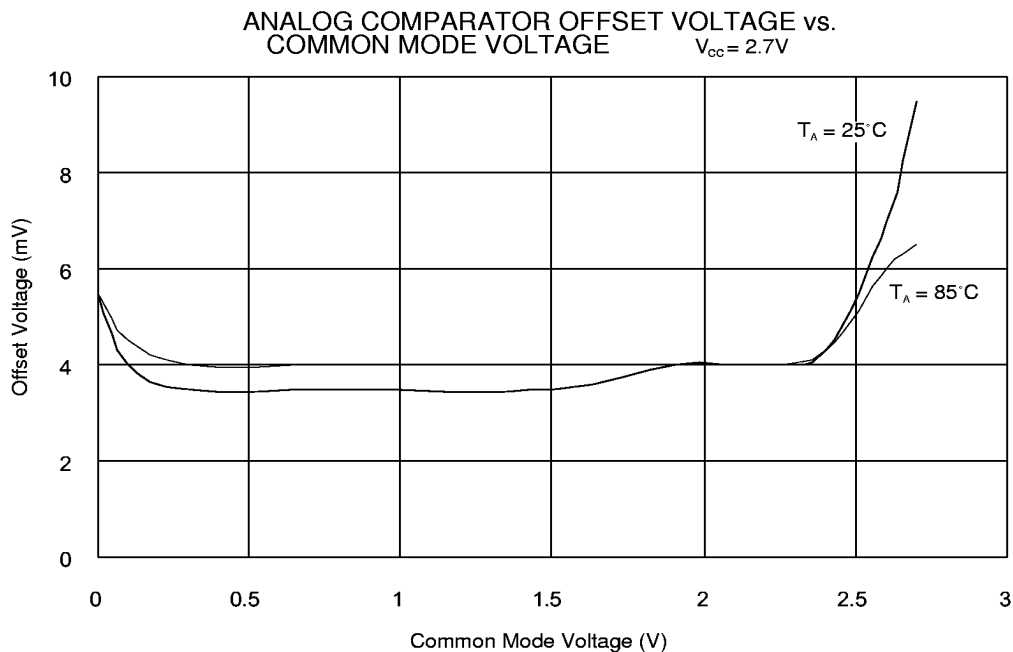
Figure 77. Analog Comparator Offset Voltage vs. Common Mode Voltage
