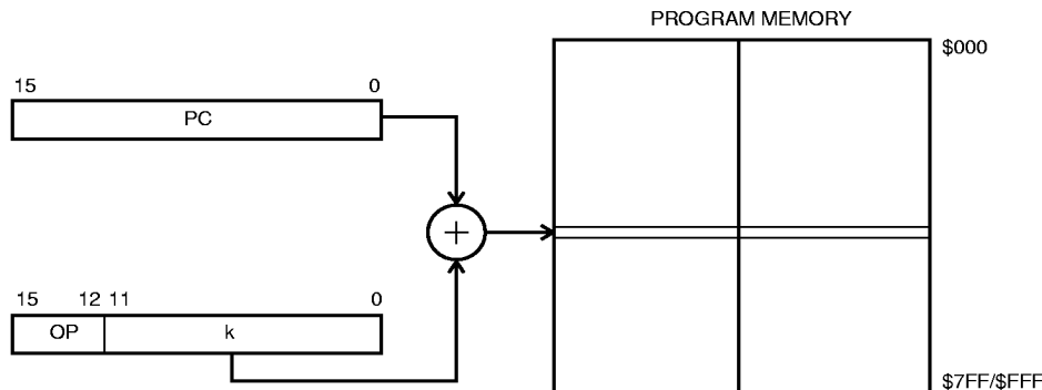
Figure 19. Relative Program Memory Addressing
