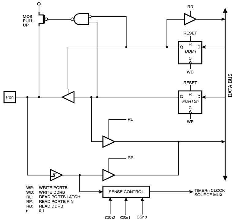
Figure 46. Port B Schematic Diagram (Pins PB0 and PB1)
