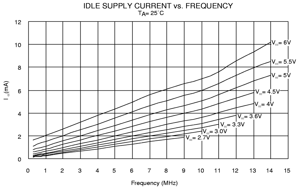
Figure 71. Idle Supply Current vs. Frequency
