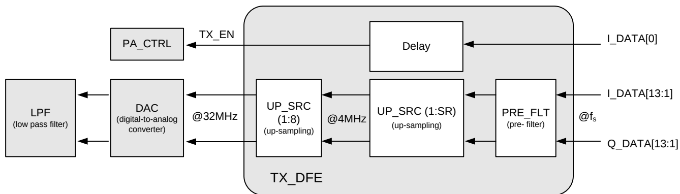
Figure 6-1. TX Up-Sampling and Filtering
