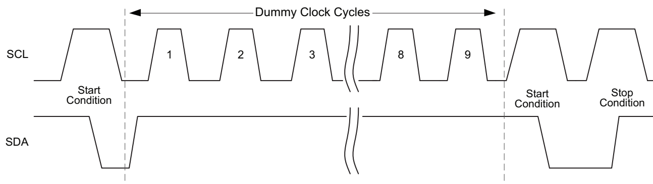
Figure 8-4. Software Reset
