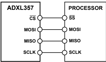
Figure 64. 4-Wire SPI Connection
