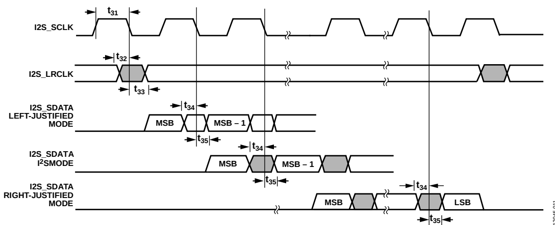
Figure 11. I2S Timing
