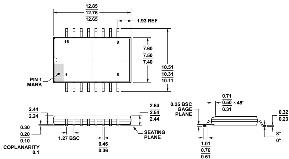
Figure 25. 16-Lead Standard Small Outline Package, with Increased Creepage [SOIC_IC] Wide Body (RI-16-2)
