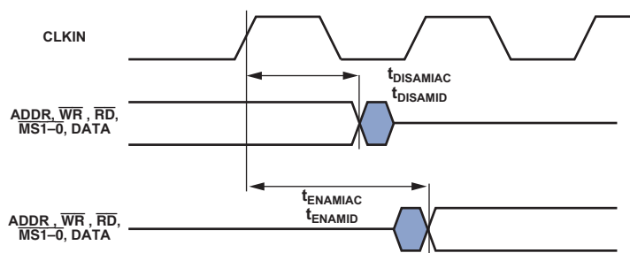
Figure 20. AMI Enable/Disable
