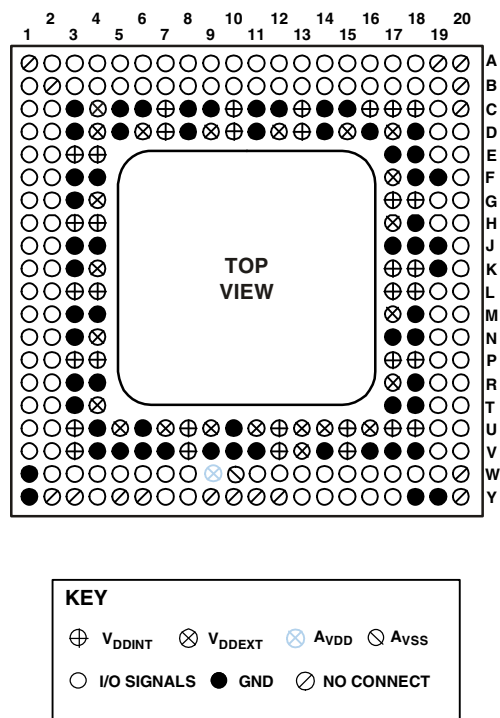
Figure 49. 256-Ball BGA_ED Ball Configuration (Top View)
