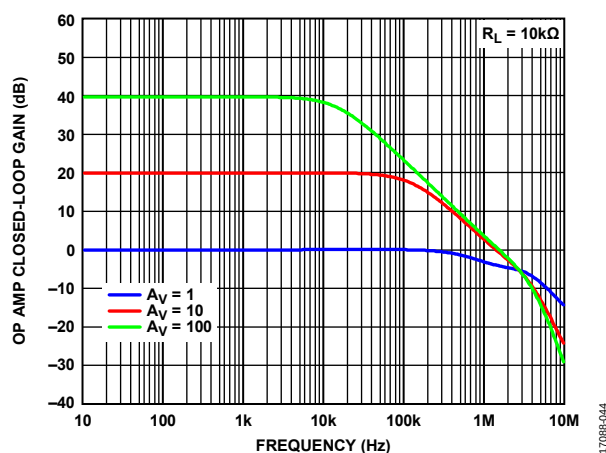
Figure 45. Op Amp Close-Loop Gain vs. Frequency
