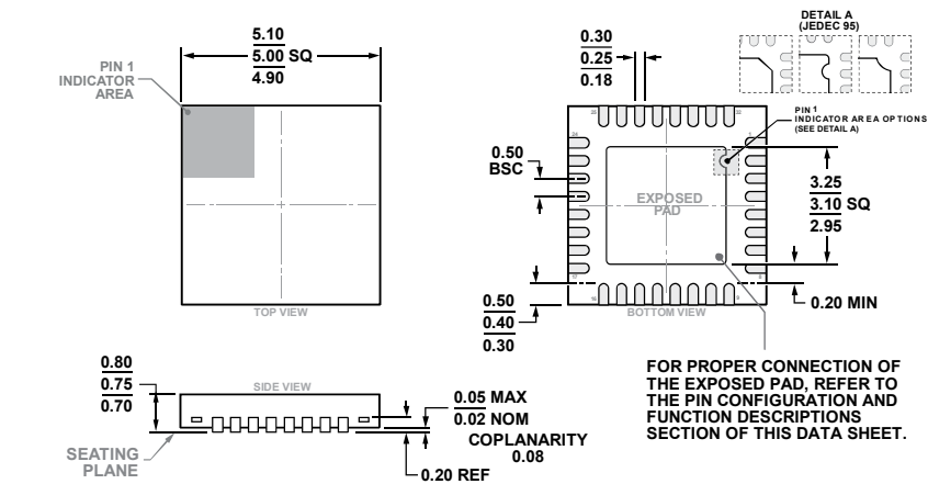
COMPLIANT TO JEDEC STANDARDS MO-220-WHHD Figure 76. 32-Lead Lead Frame Chip Scale Package [LFCSP] 5 mm × 5 mm Body and 0.75 mm Package Height (CP-32-7)
