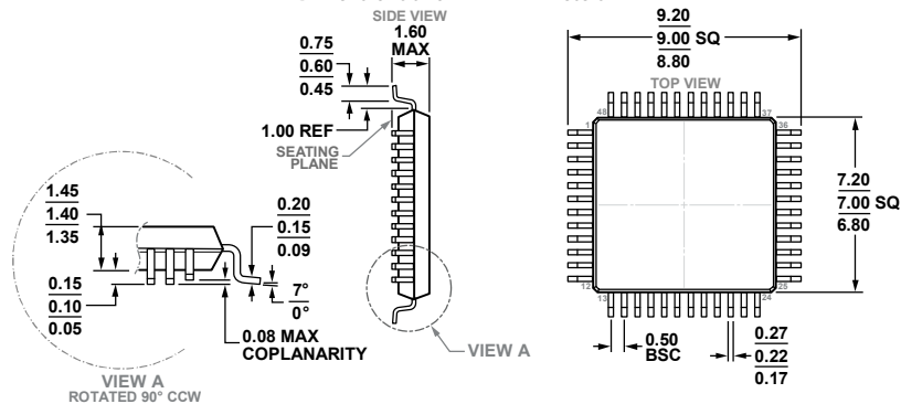
COMPLIANT TO JEDEC STANDARDS MS-026-BBC Figure 77. 48-Lead Low Profile Quad Flat Package [LQFP] (ST-48)
