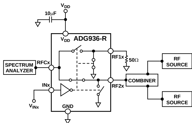
Figure 25. IP_3
