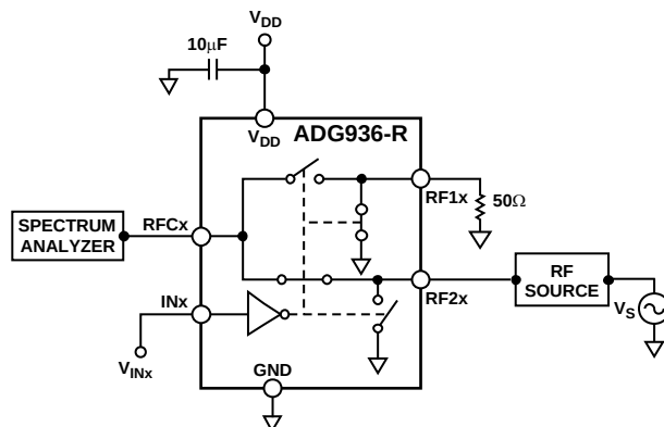
Figure 26. P_{-1dB}
