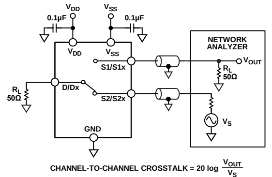
Figure 42. Channel-to-Channel Crosstalk
