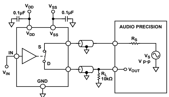
Figure 37. THD + N
