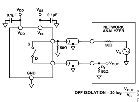
Figure 34. Off Isolation
