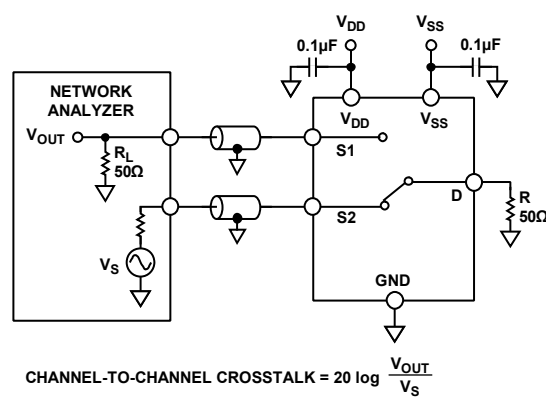
Figure 36. Channel-to-Channel Crosstalk
