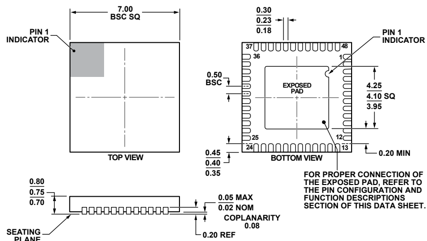
Figure 52. 48-Lead Lead Frame Chip Scale Package [LFCSP_WQ]
