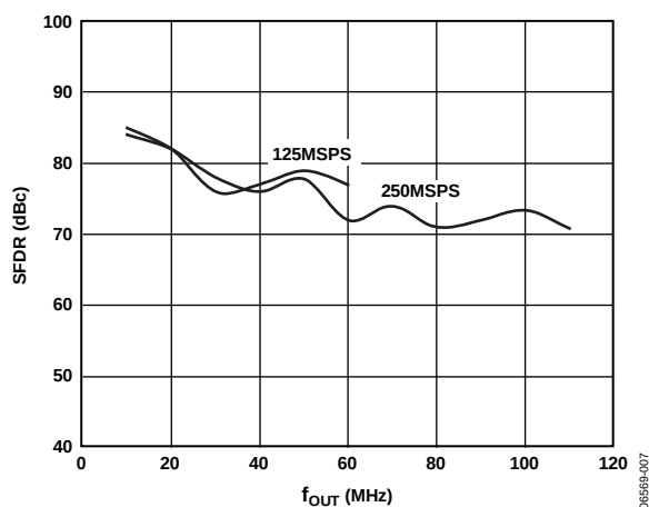
Figure 7. AD9741 SFDR vs. f_{OUT} , Normal Mode
