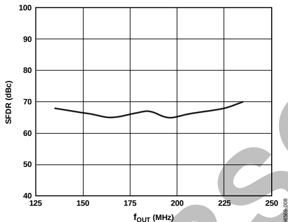
Figure 8. AD9741 SFDR vs. f_{OUT} , Mix Mode, 250 MSPS
