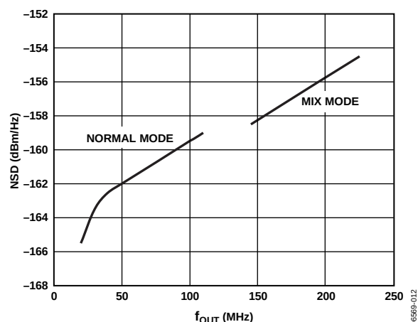
Figure 12. AD9741 NSD vs. f_{OUT} , Single Carrier WCDMA, 245.76 MSPS
