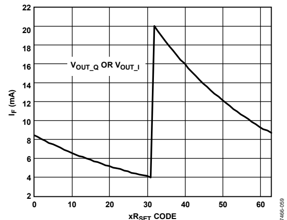
Figure 98. Effect of xR_{SET} Code
