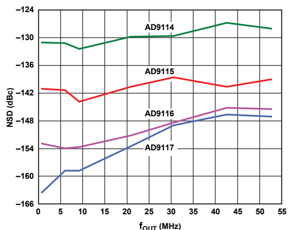
Figure 40. NSD at 20 mA vs. f_{OUT} , 3.3 V
