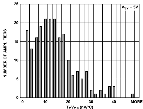
Figure 7. T_C V_{OS} at V_{SY} = 5V
