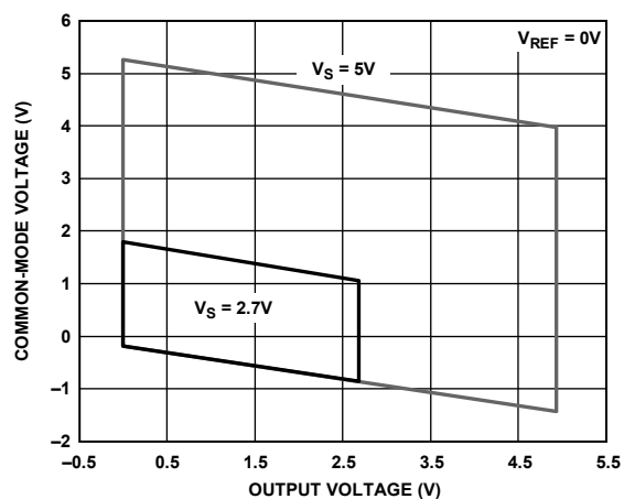
Figure 17. Input Common-Mode Voltage vs. Output Voltage, 5 V and 2.7 V Supplies, V_{REF} = 0V , G = 2
