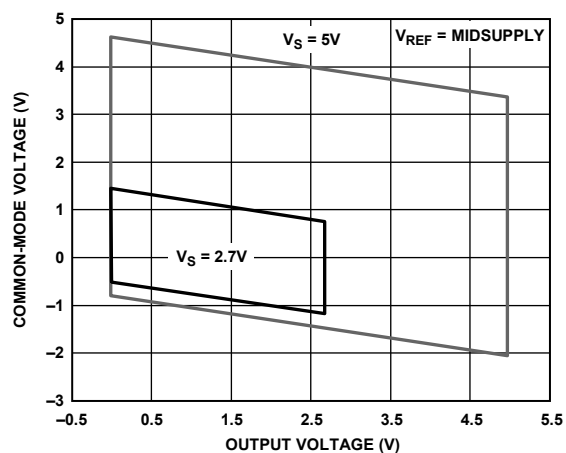
Figure 16. Input Common-Mode Voltage vs. Output Voltage, 5 V and 2.7 V Supplies, V_{REF} = \text{Midsupply} , G = 2
