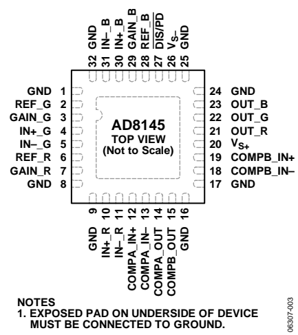
Figure 3. Pin Configuration
