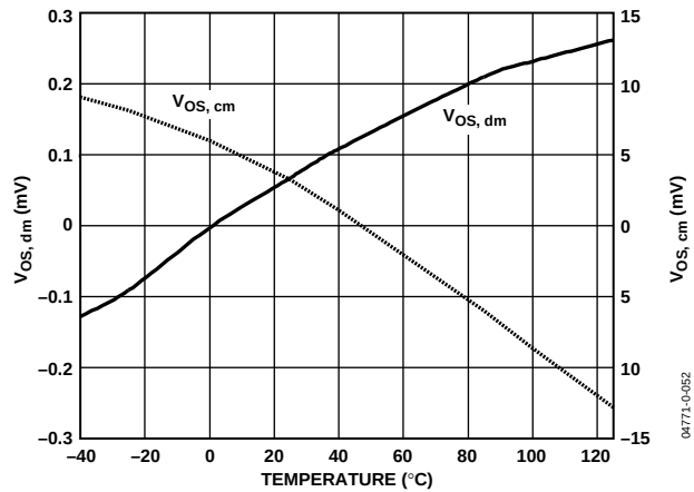
Figure 47. Offset Voltage vs. Temperature
