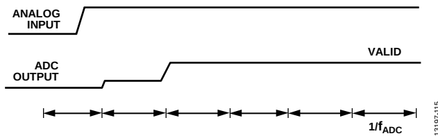
Figure 109. Step Change on the Analog Input, \text{Sinc}^3 + \text{Sinc}^1 Filter
