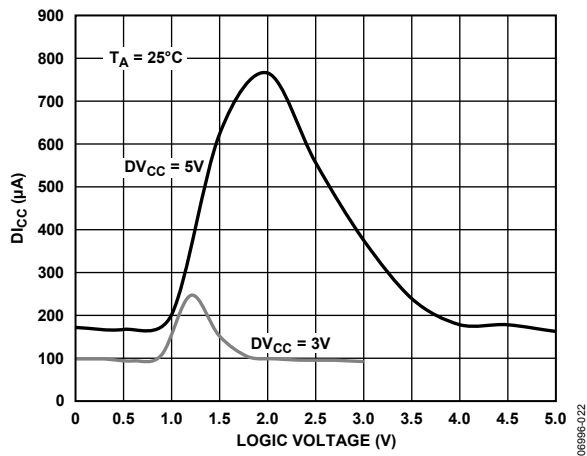
Figure 7. D_{ICE} vs. Logic Input Voltage
