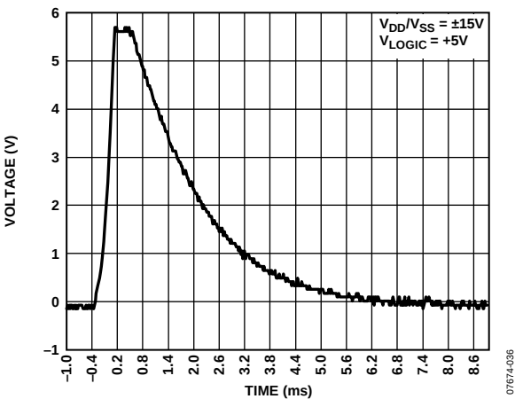
Figure 54. V_{EXT\_CAP} Waveform While Reading Fuse Or Calibration
