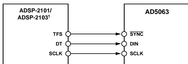
Figure 30. AD5063 to ADSP-2101/ADSP-2103 Interface
