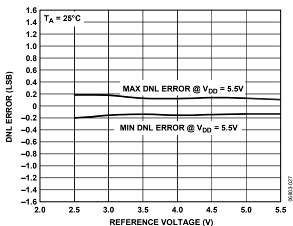
Figure 16. DNL vs. Reference Input Voltage
