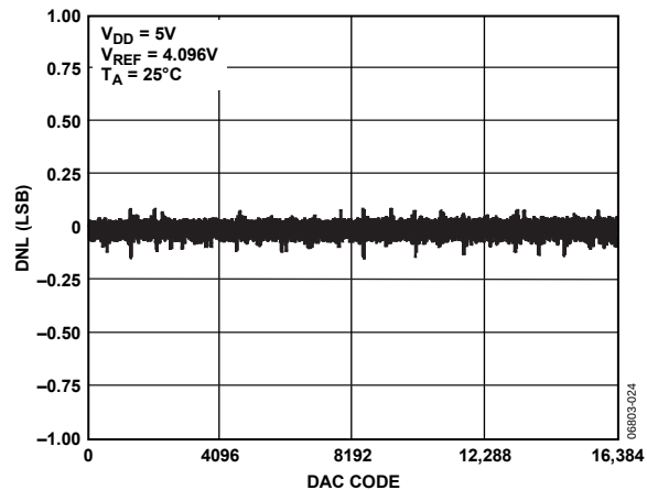
Figure 13. AD5024 DNL
