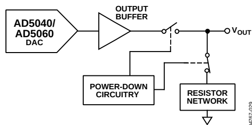
Figure 44. Output Stage During Power-Down
