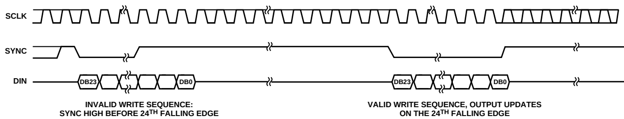
Figure 43. AD5060 SYNC Interrupt Facility
