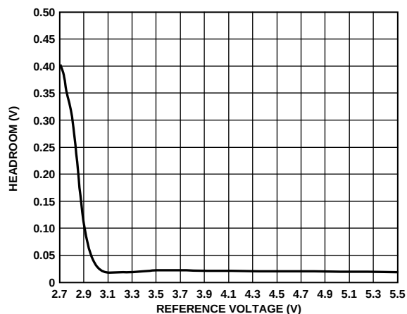
Figure 26. V_{DD} Headroom vs. Reference Voltage
