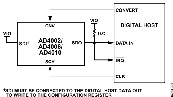
Figure 55. \overline{\text{CS}} Mode, 3-Wire with Busy Indicator Connection Diagram
