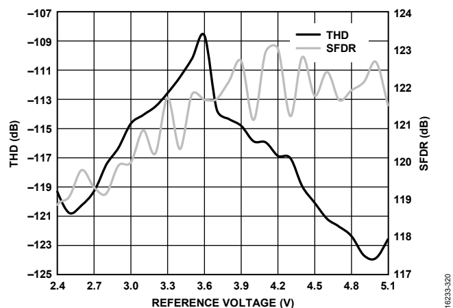
Figure 21. THD and SFDR vs. Reference Voltage, f_{IN} = 1 \text{ kHz}
