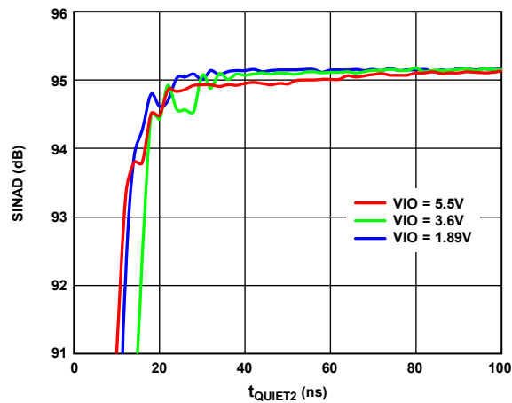
Figure 24. SINAD vs. t_{\text{QUIET2}}
