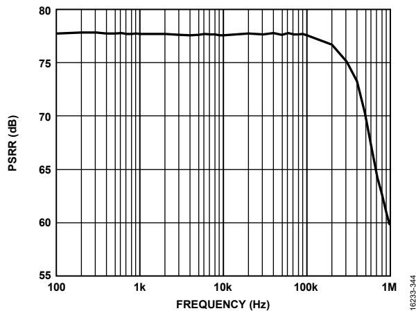
Figure 32. PSRR vs. Frequency, V_{DD} = 1.8\text{ V} , V_{IO} = 3.3\text{ V} , V_{REF} = 5\text{ V} , T_A = 25^\circ\text{C}
