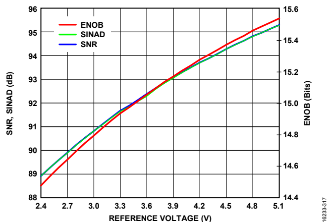
Figure 18. SNR, SINAD, and ENOB vs. Reference Voltage, f_{IN} = 1 \text{ kHz}
