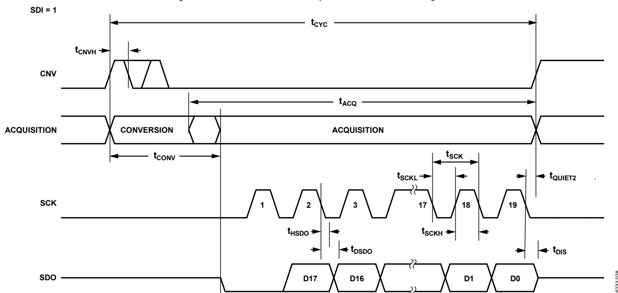
Figure 56. \overline{\text{CS}} Mode, 3-Wire with Busy Indicator Serial Interface Timing Diagram (Status Bits Not Shown)
