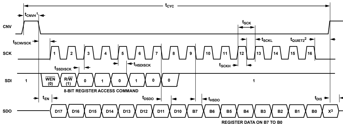
Figure 47. Register Read Timing Diagram
