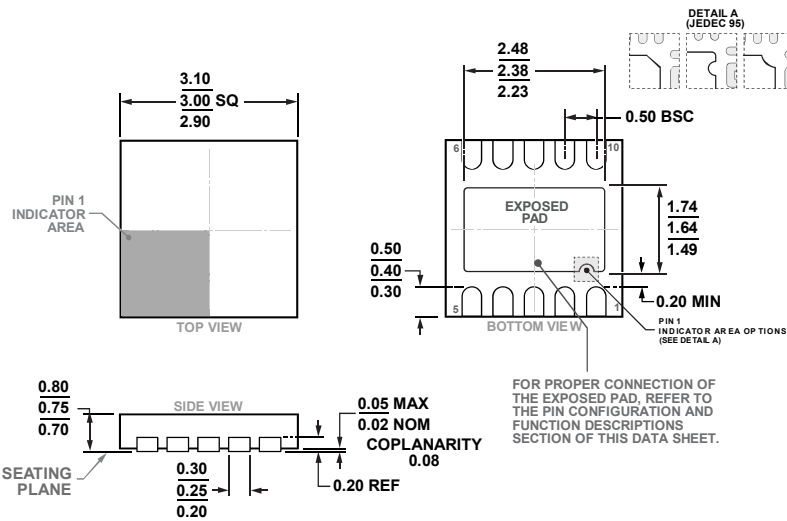
Figure 68. 10-Lead Lead Frame Chip Scale Package [LFCSP] 3 mm × 3 mm Body and 0.75 mm Package Height (CP-10-9) Dimensions shown in millimeters
