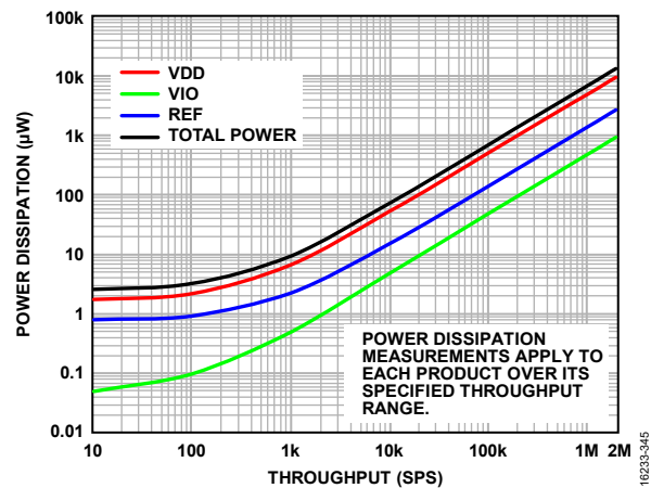
Figure 34. Power Dissipation vs. Throughput, V_{DD} = 1.8\text{ V} , V_{IO} = 1.8\text{ V} , V_{REF} = 5\text{ V}
