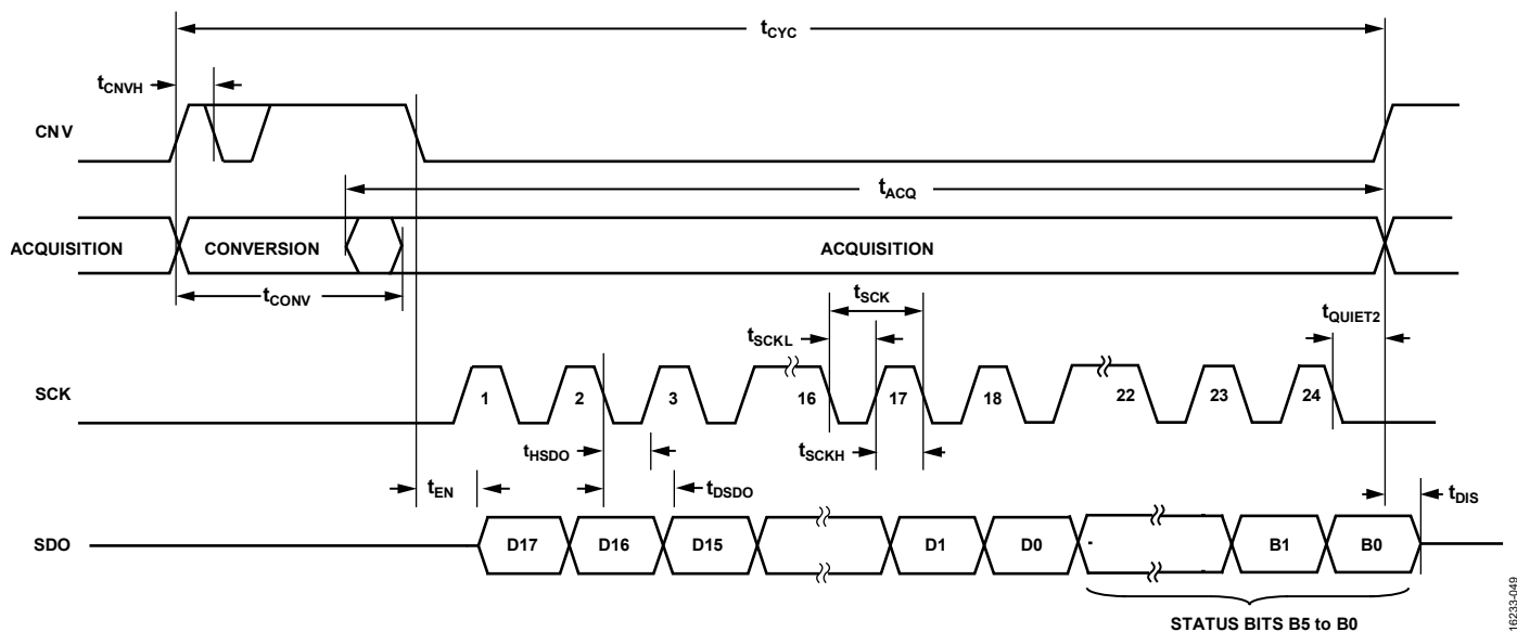
Figure 50. \overline{\text{CS}} Mode, 3-Wire Without Busy Indicator Serial Interface Timing Diagram, Including Status Bits
