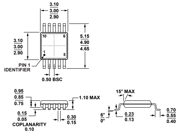
Figure 67. 10-Lead Mini Small Outline Package [MSOP] (RM-10) Dimensions shown in millimeters
