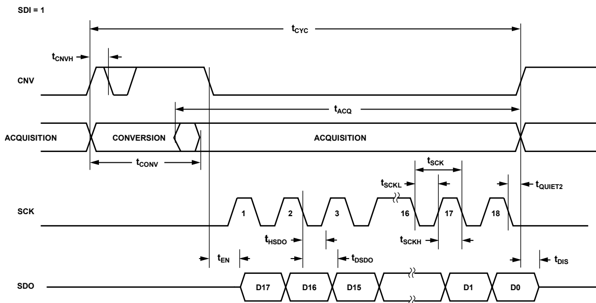
Figure 54. CS Mode, 3-Wire Without the Busy Indicator Serial Interface Timing Diagram (Status Bits Not Shown)
