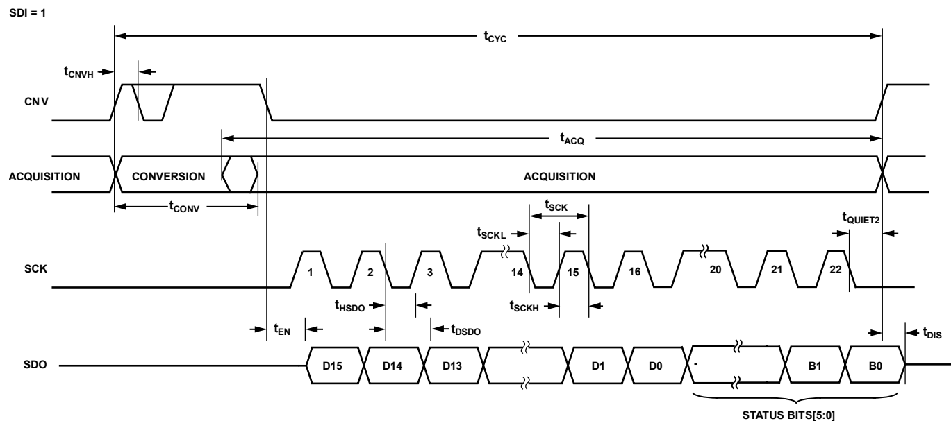
Figure 49. \overline{CS} Mode, 3-Wire Without Busy Indicator Serial Interface Timing Diagram, Including Status Bits
