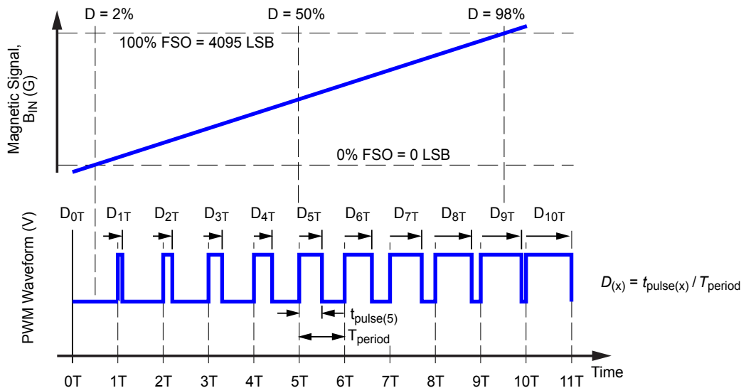
Figure 11: PWM Mode Duty-Cycle-Based Waveform PWM mode outputs a duty-cycle-based waveform that can be read by the external controller as a cumulatively changing continuous voltage.
