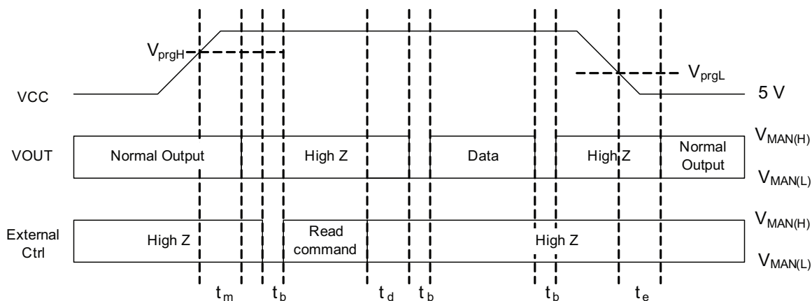
Figure 28: Read Request
