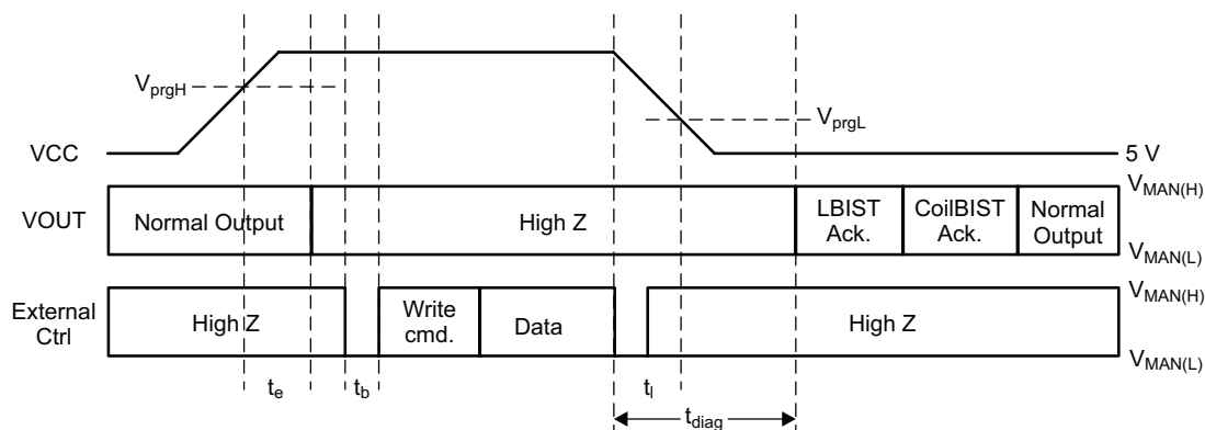
Figure 29: BIST Request
