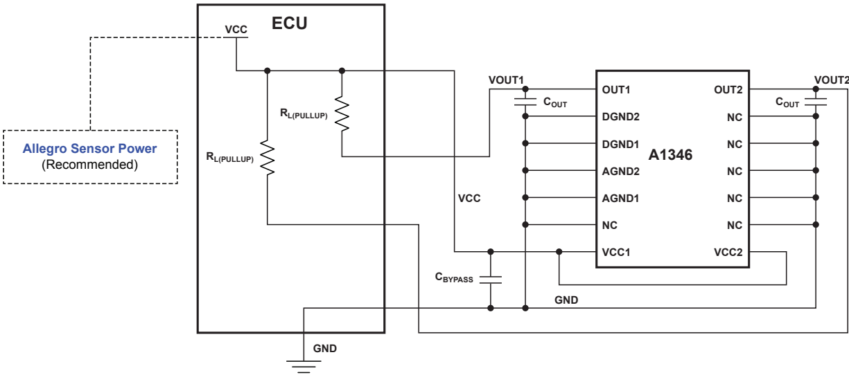
Figure 2: Typical Application Circuit Typical C BYPASS = 0.1 μF and C OUT = 1.5 nF
