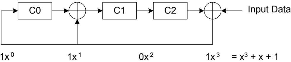
Figure 32: CRC Calculation
