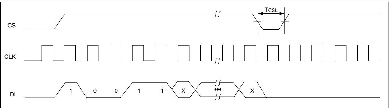
FIGURE 3-5: EWEN TIMING
