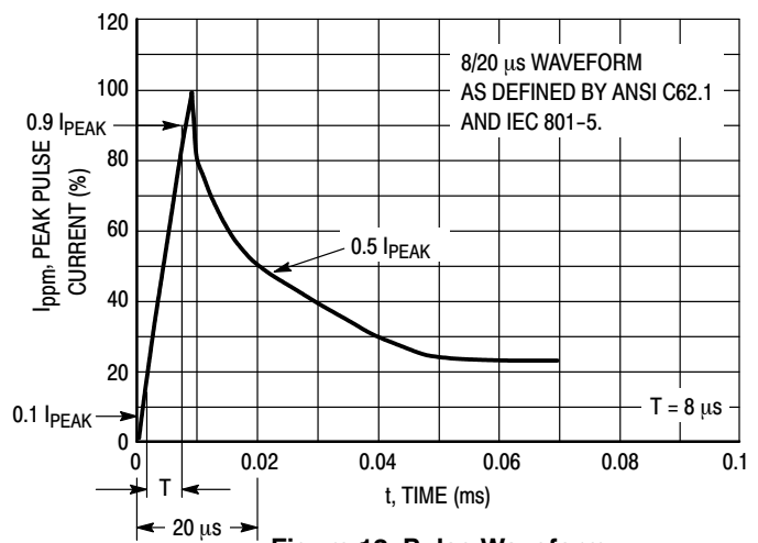
Figure 12. Pulse Waveform
