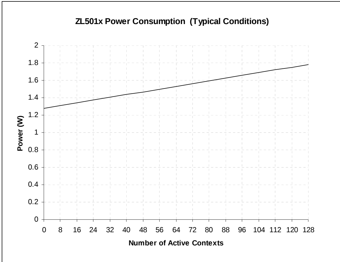
Figure 49 - ZL50110/11/12/14 Power Consumption Plot
