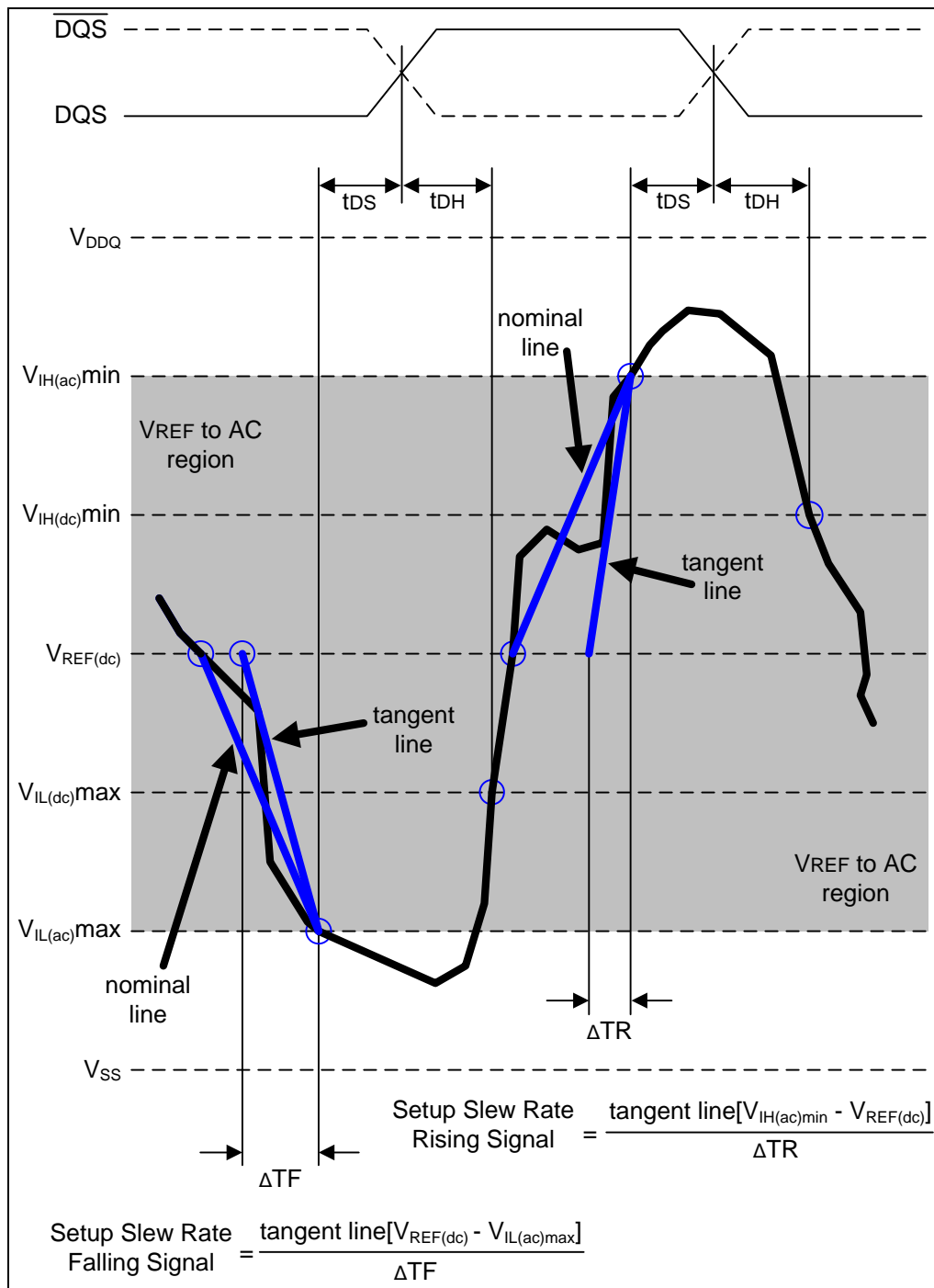
Figure 25 – Illustration of tangent line for t_{\text{DS}} (differential \overline{\text{DQS}} , \text{DQS} )
