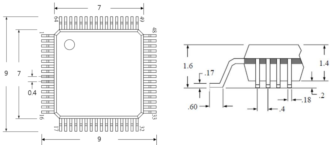
Figure 83. Package Dimension Information
