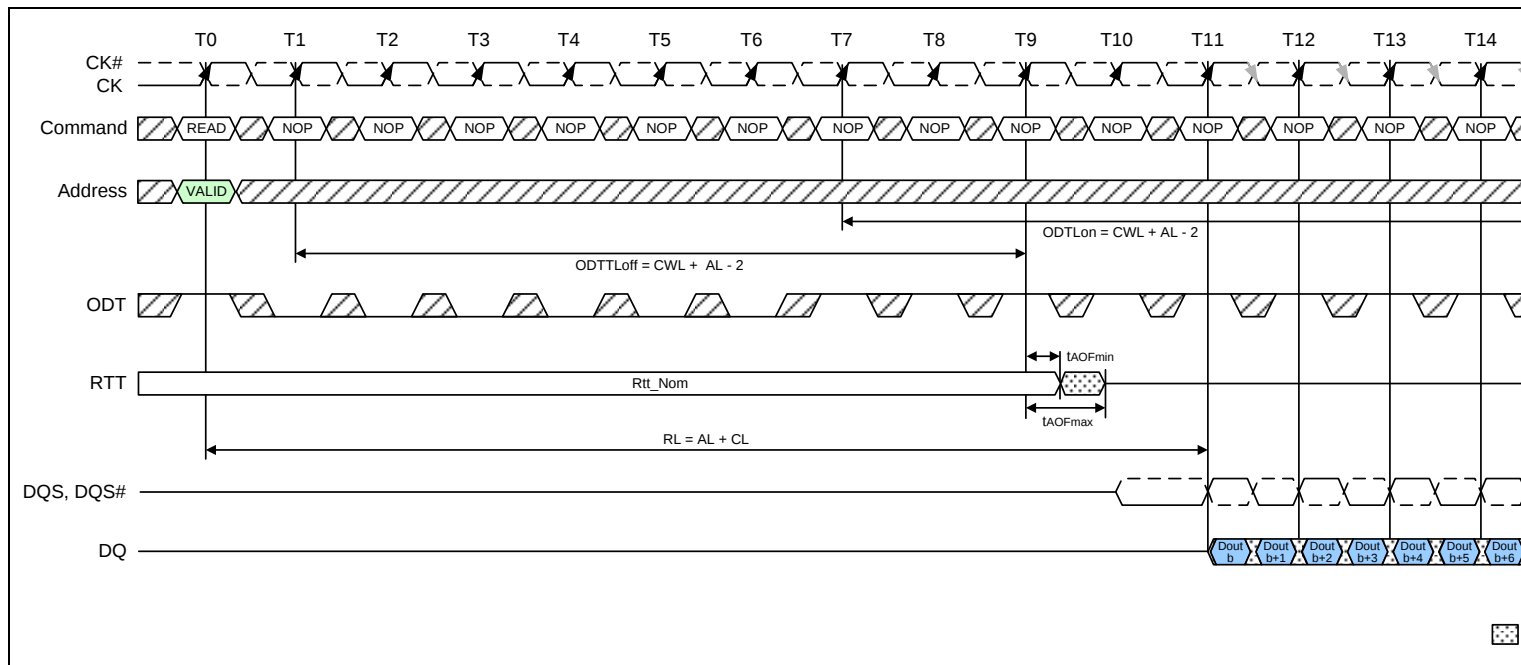
Figure 76 – ODT must be disabled externally during Reads by driving ODT low. (CL = 6; AL = CL - 1 = 5; RL = AL + CL = 11; CWL = 5; ODTLo = CWL + AL - 2 = 8; ODTLo = CWL + AL - 2 = 8)
