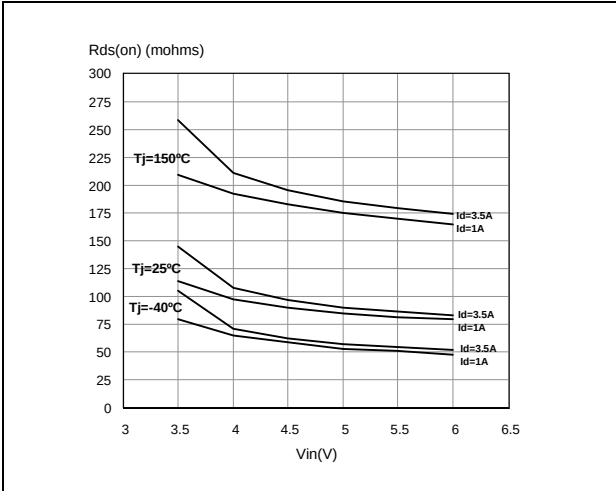
Figure 13. Static drain-source on resistance vs input voltage (part 1/2)
