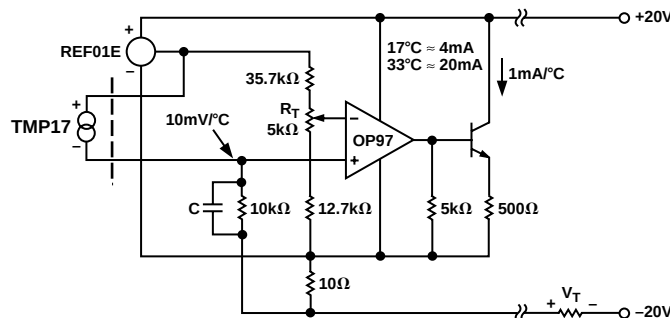
Figure 10. Temperature to 4–20 mA Current Transmitter
