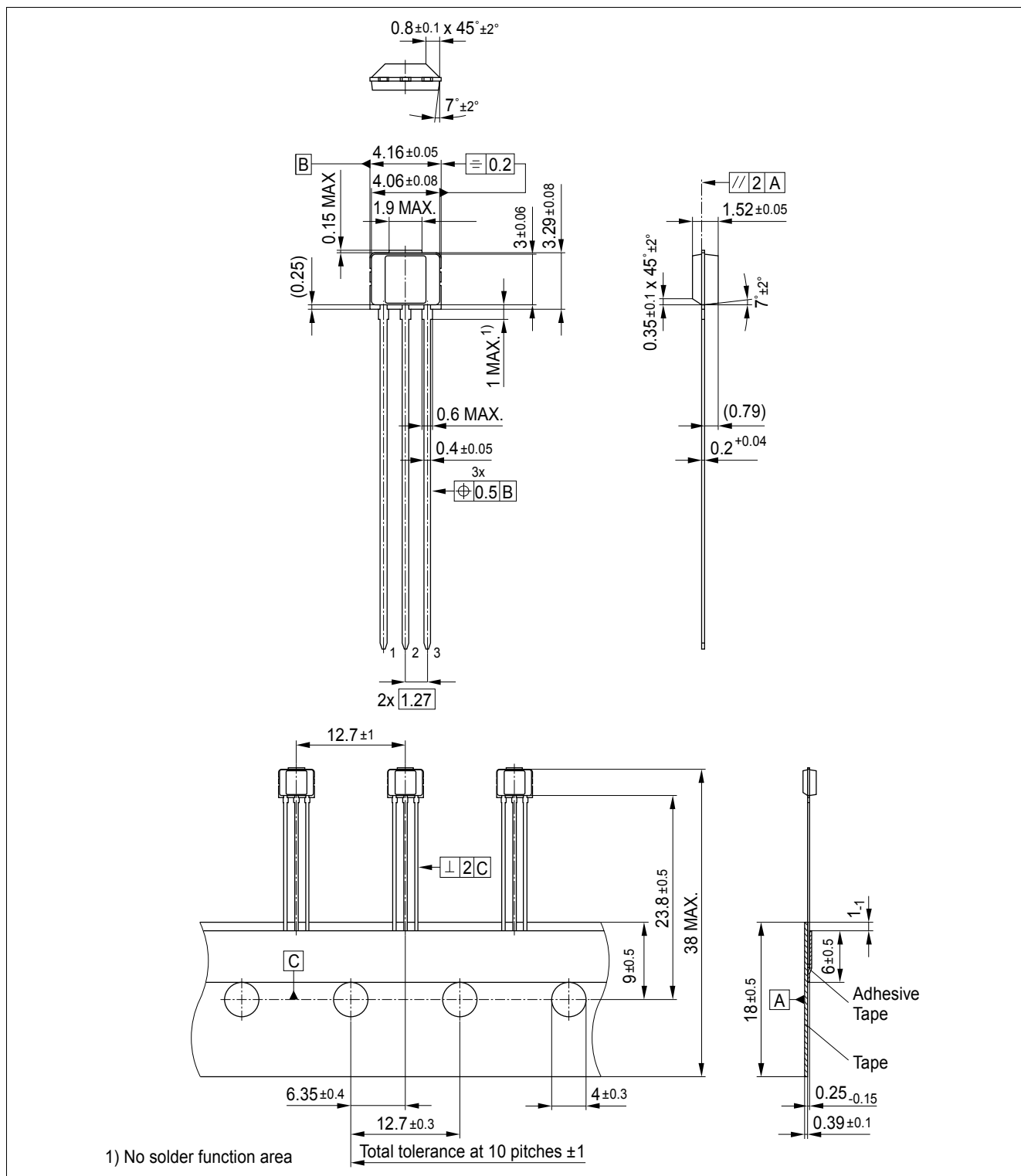
Figure 4-4 PG-SSO-3-2 Package Outline (All Dimensions in mm)
