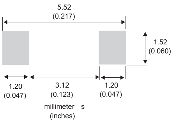
Figure 15. SMA Flat recommended footprint in mm (inches)
