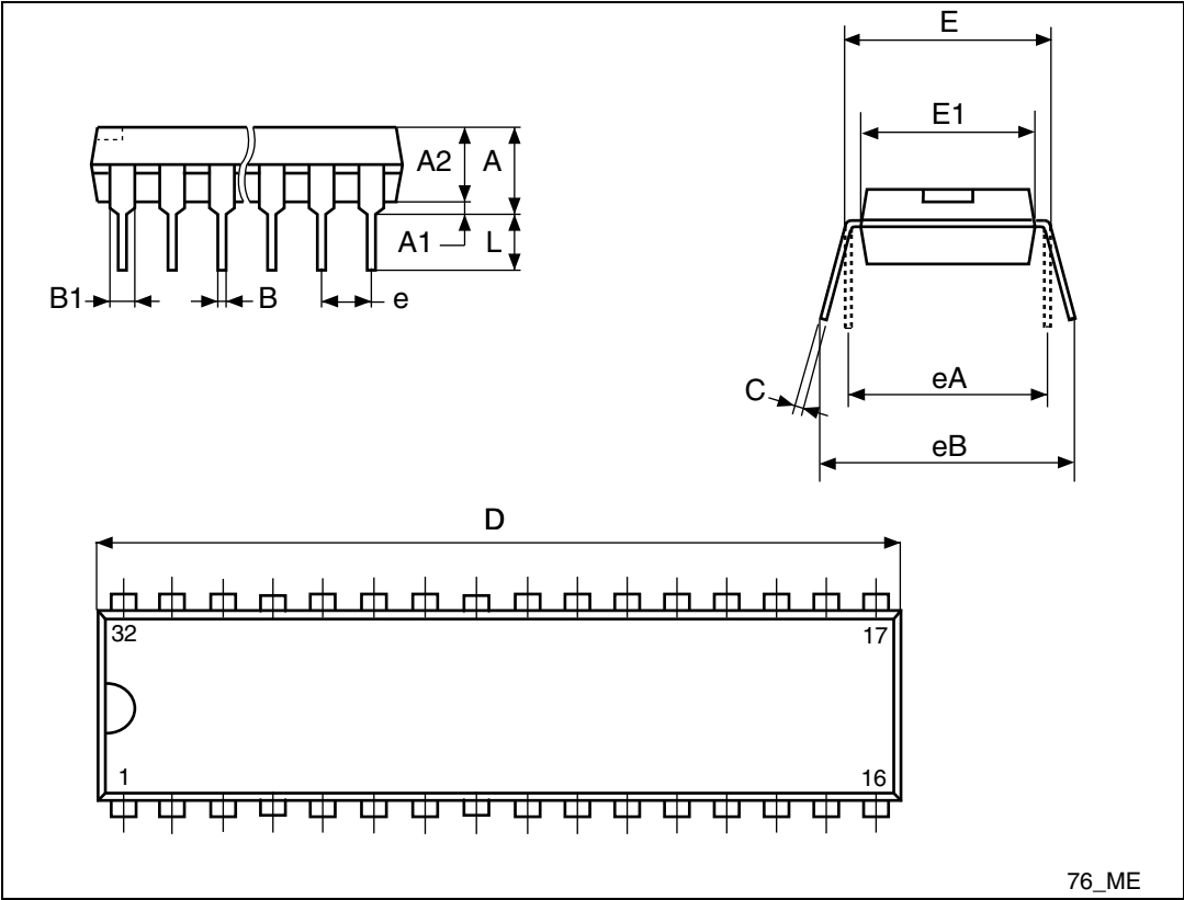
Figure 54. SDIP32 package outline
