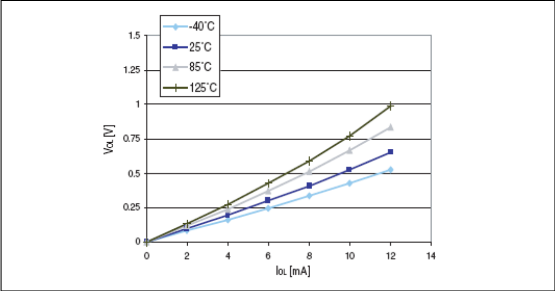
Figure 29. Typ. V_{OL} @ V_{DD} = 3.3\text{ V} (high sink ports)
