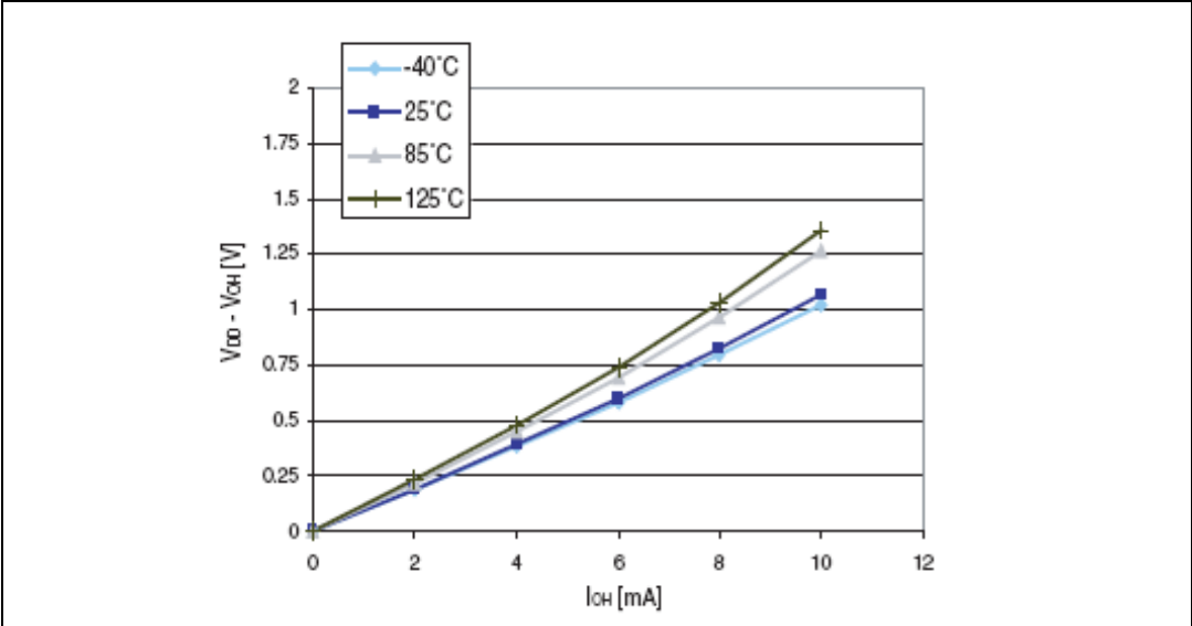
Figure 30. Typ. V_{DD} - V_{OH} @ V_{DD} = 5\text{ V} (standard ports)
