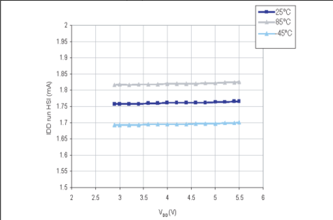
Figure 13. Typ. I_{DD(RUN)} vs V_{DD} , HSI RC osc, f_{CPU} = 16\text{ MHz}
