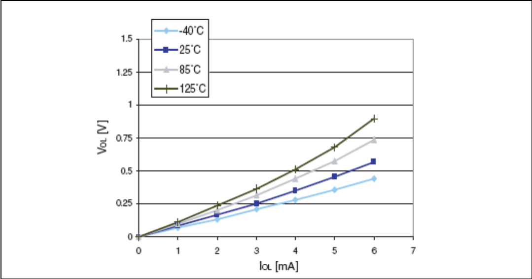
Figure 25. Typ. V_{OL} @ V_{DD} = 3.3\text{ V} (standard ports)
