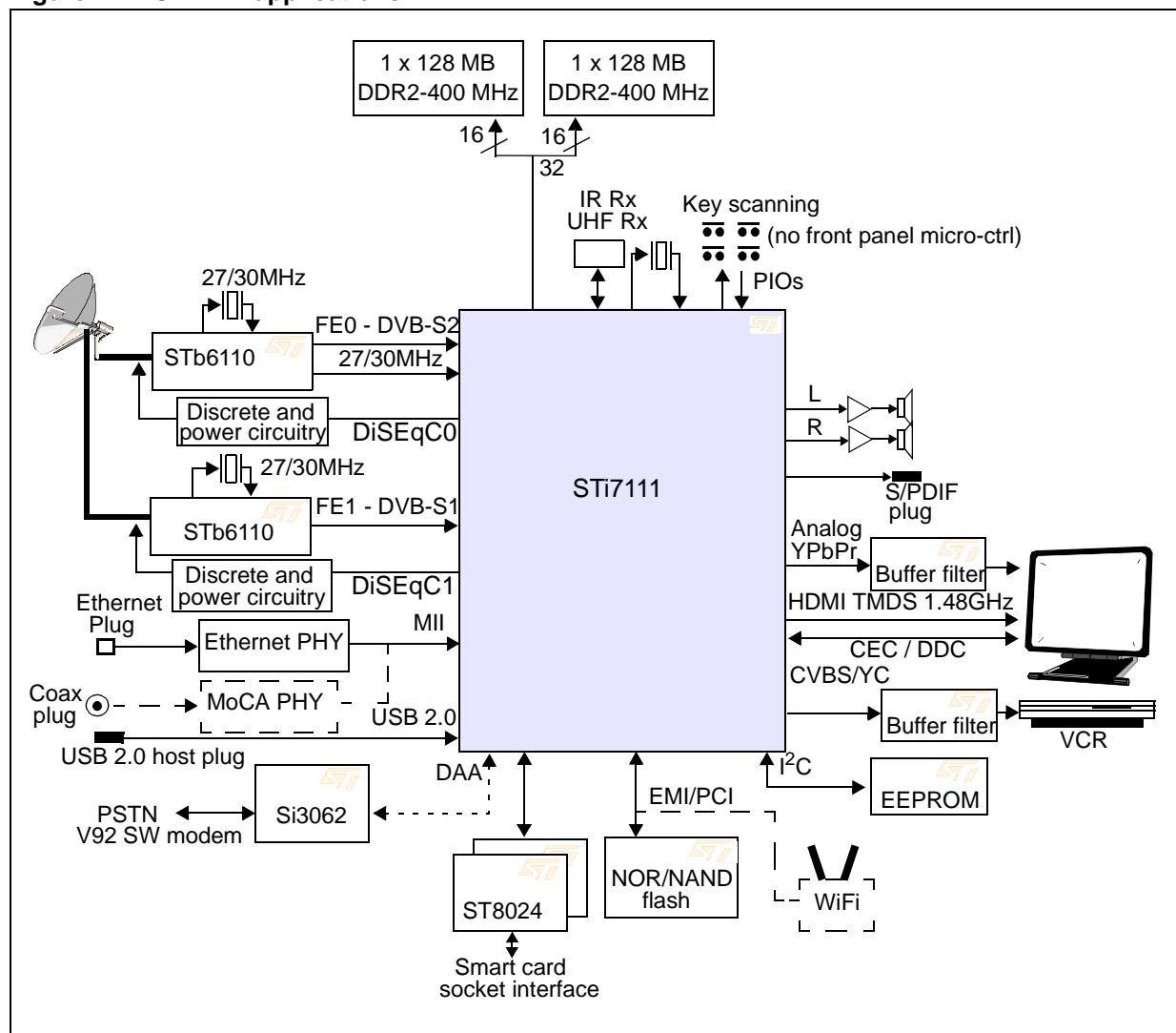
Figure 1. STi7111 applications
