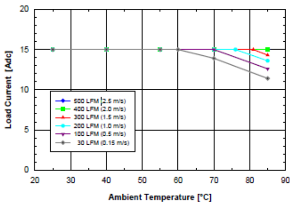
Fig. 2.0V.3: Available load current vs. ambient air
