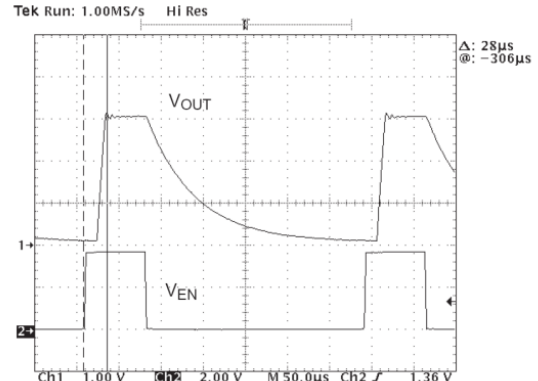
Fig. 5: Turn-On Time, R_{LOAD}=50\Omega (60mA)
