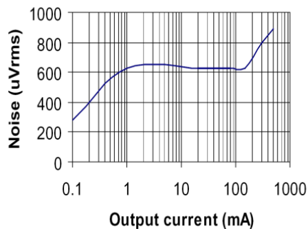
Fig. 20: Output Noise, C_{BYP} = \text{open}
