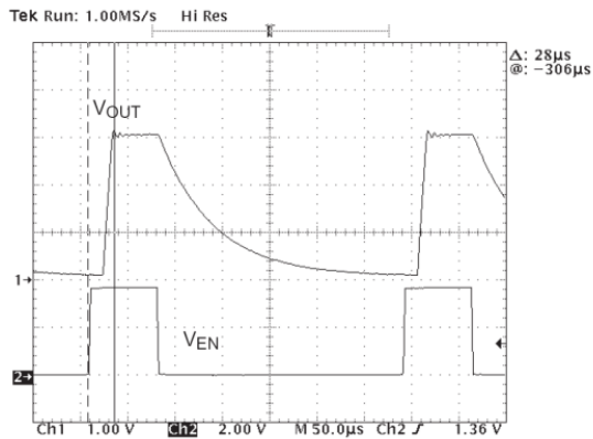
Fig. 6: Turn-Off Time, R_{LOAD}=6\Omega (500mA)
